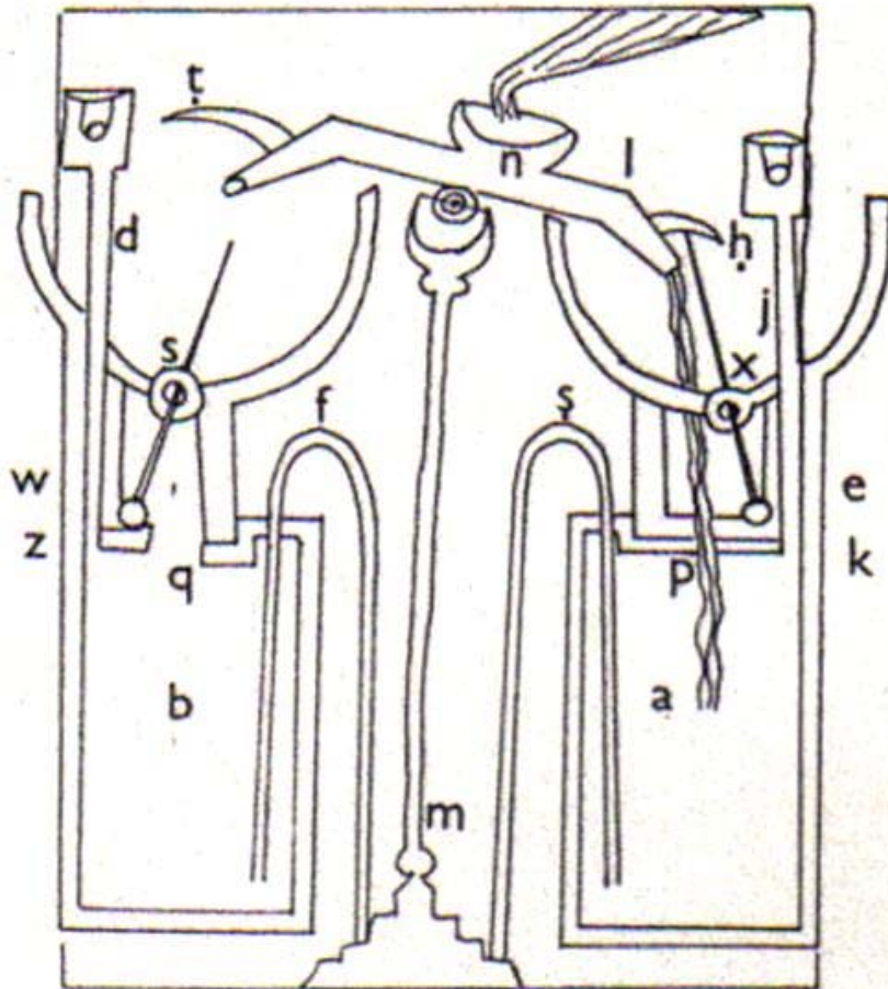
Figure 6: Diagram of the perpetual flute (al-Jazari, 1206/1974: 177)
