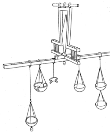
Figure 4. Al-Khŷzinŷ's balance in Seyyed Hossein Nasr. Islamic Science an Illustrated Study . Kent 1976 (The image was introduced by the editor).
