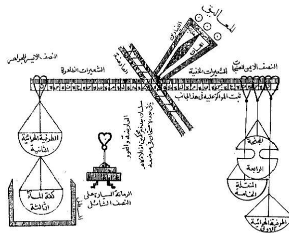
Al-mizan al-jami' (the universal balance) of al-Khazini, as depicted in Al-Khazini, Kitab mizan al-hikma , Hyderabad, 1359 (1940), p. 103.
